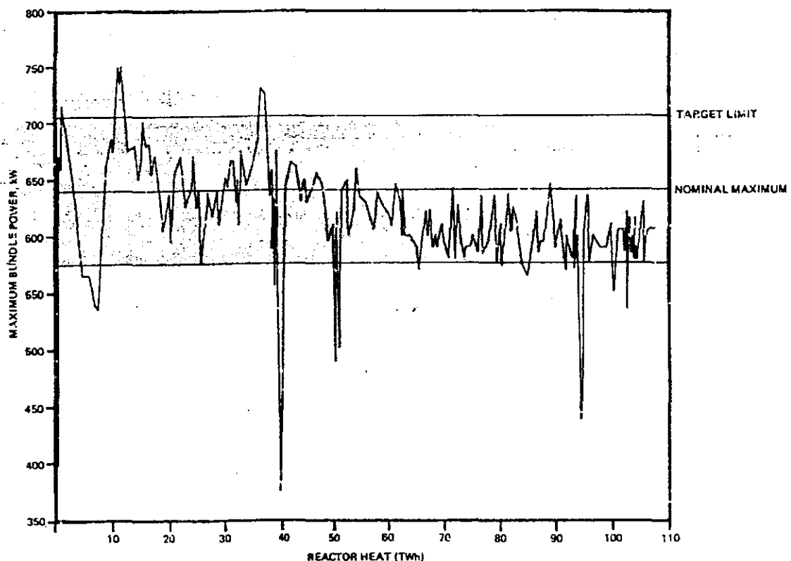
FIGURE 6.1 PICKERING PICKERING UNIT1, MAXIMUM BUNDLE POWER
