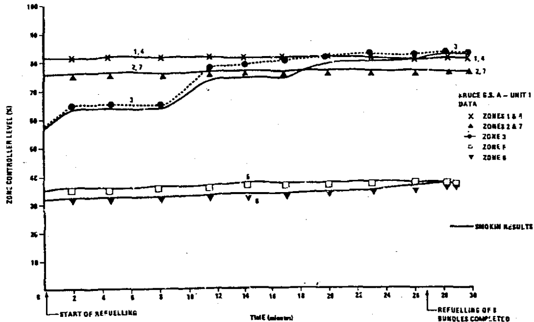
FIGURE 6.7 ZONE CONTROLLER LEVEL TRANSIENT FOR SINGLE CHANNEL REFUELLING (ZONE 1 TO 7)
