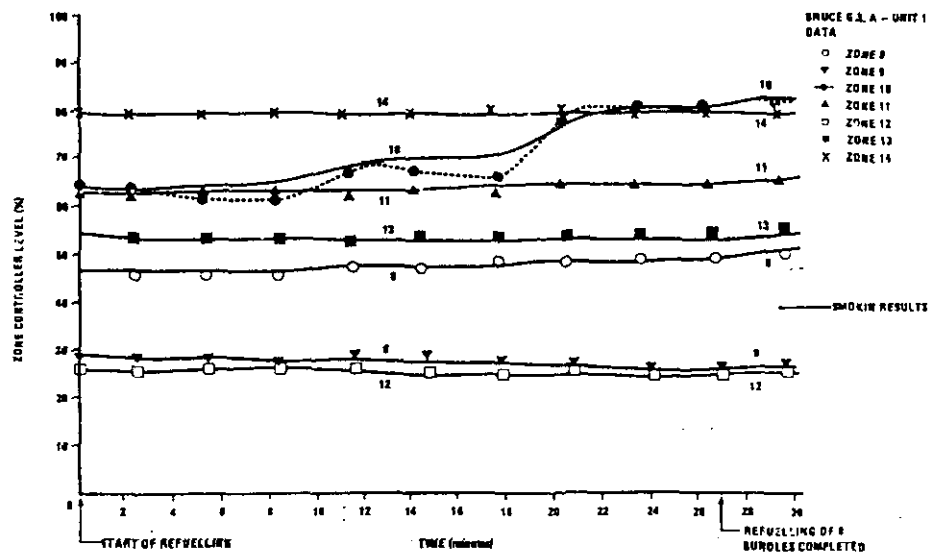
FIGURE 6.8 ZONE CONTROLLER LEVEL TRANSIENT FOR SINGLE CHANNEL REFUELLING (ZONE 8 TO 14)
