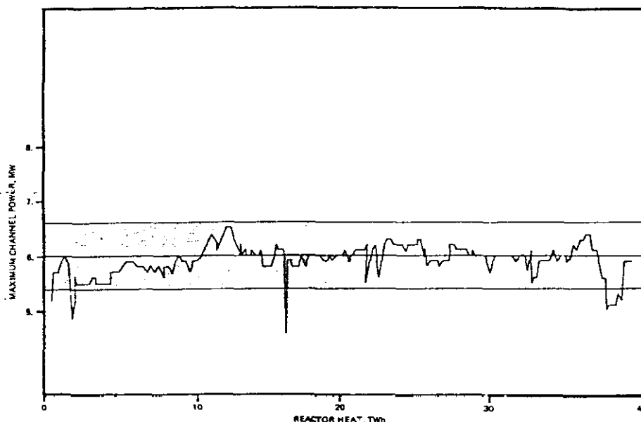
FIGURE 6.10 BRUCE UNIT 1, MAXIMUM BUNDLE POWER
